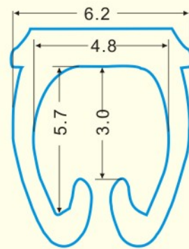
规格: 2.5mm 2
