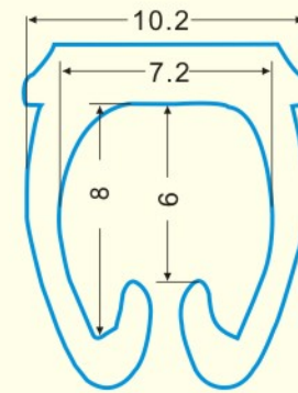
规格: 6mm 2
